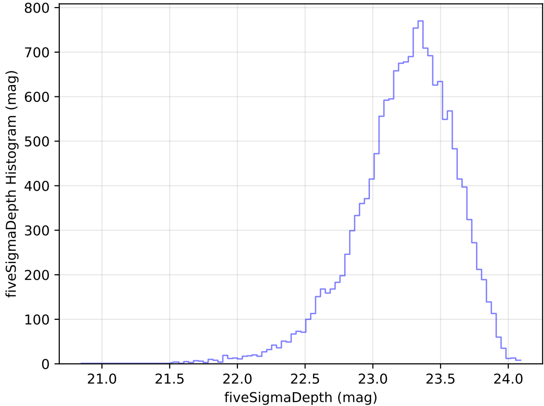
too_elab_heavy_r32_d2_griz_v3.4_10yrs Yr 1 u band: fiveSigmaDepth Histogram
