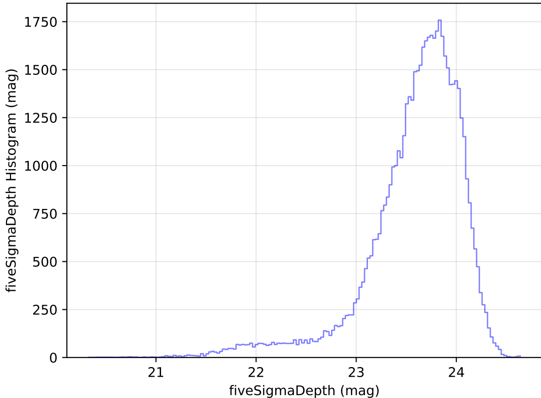
too_elab_heavy_r32_d2_griz_v3.4_10yrs Yr 1 i band: fiveSigmaDepth Histogram
