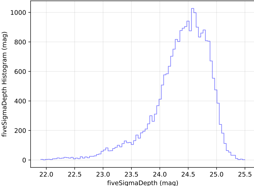
too_elab_heavy_r32_d2_griz_v3.4_10yrs Yr 1 g band: fiveSigmaDepth Histogram
