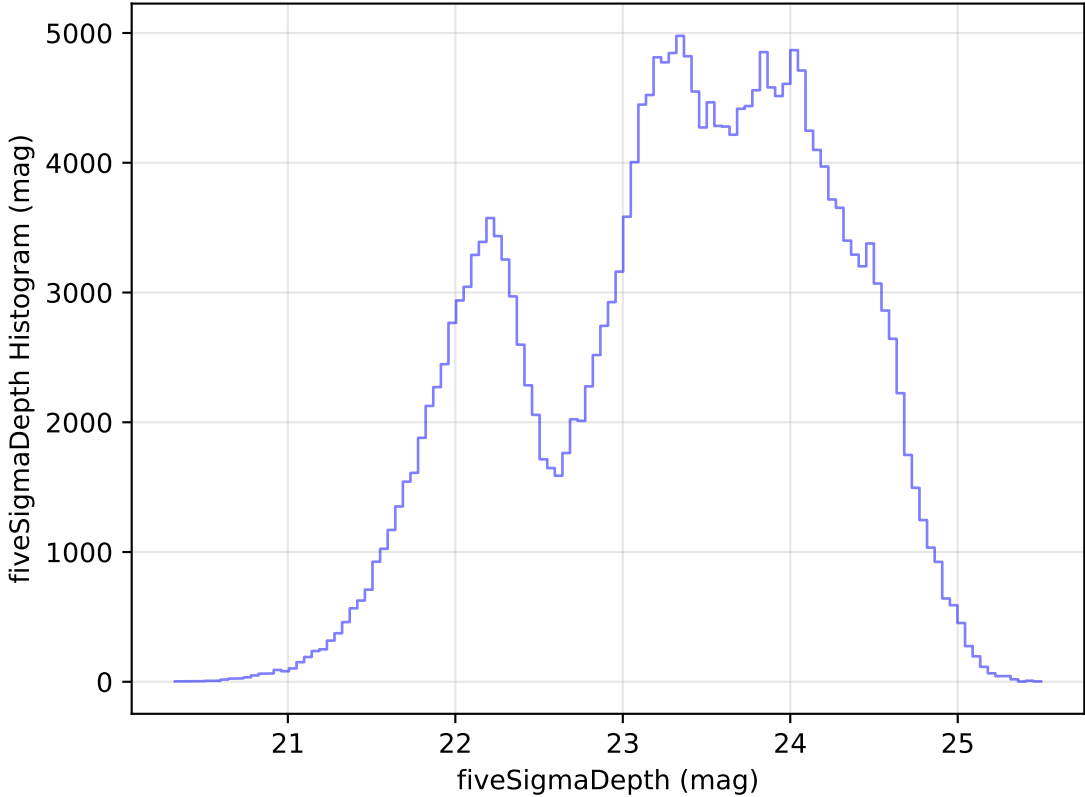
too_elab_heavy_r32_d2_griz_v3.4_10yrs Yr 1 all bands: fiveSigmaDepth Histogram
