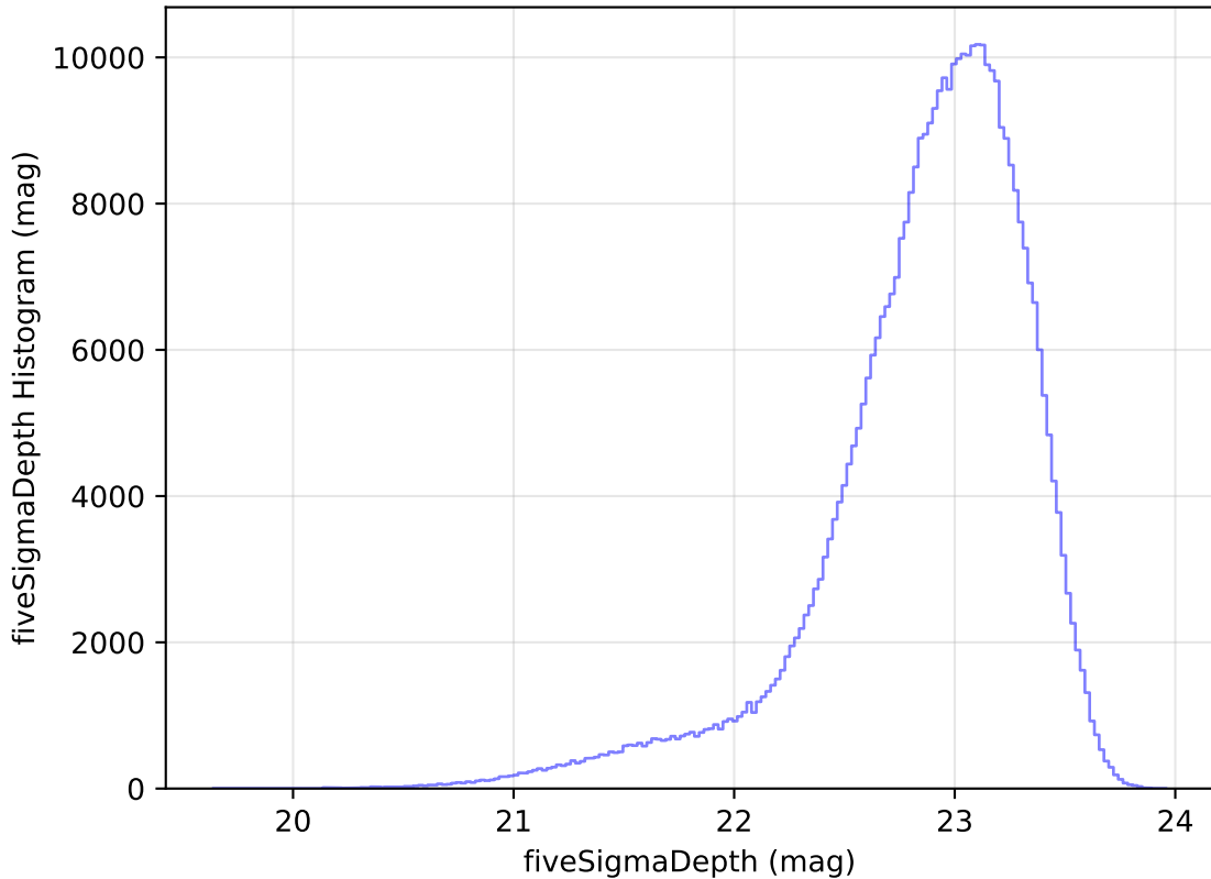
too_elab_heavy_r32_d2_griz_v3.4_10yrs WFD z band: fiveSigmaDepth Histogram
