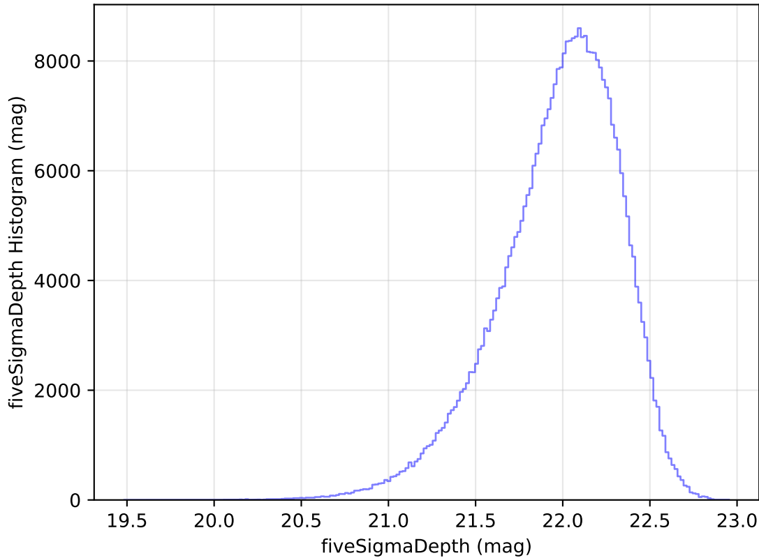
too_elab_heavy_r32_d2_griz_v3.4_10yrs WFD y band: fiveSigmaDepth Histogram
