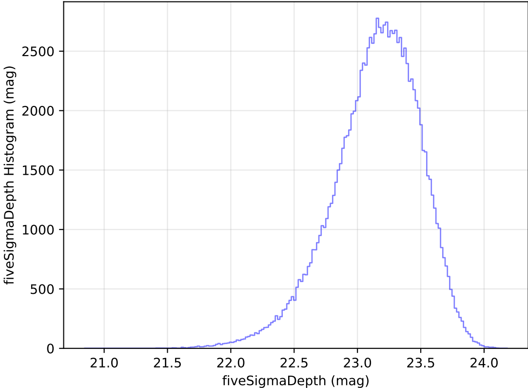
too_elab_heavy_r32_d2_griz_v3.4_10yrs WFD u band: fiveSigmaDepth Histogram
