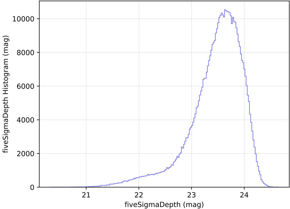
too_elab_heavy_r32_d2_griz_v3.4_10yrs WFD i band: fiveSigmaDepth Histogram
