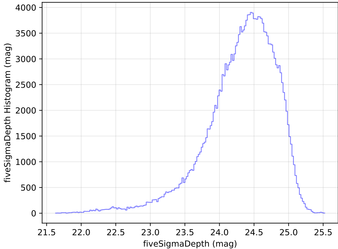
too_elab_heavy_r32_d2_griz_v3.4_10yrs WFD g band: fiveSigmaDepth Histogram
