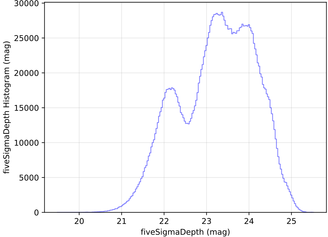
too_elab_heavy_r32_d2_griz_v3.4_10yrs WFD all bands: fiveSigmaDepth Histogram
