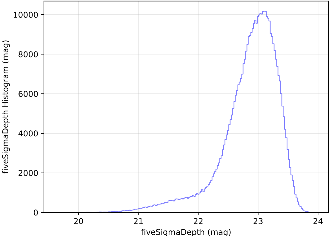
too_elab_heavy_r32_d2_griz_v3.4_10yrs All sky z band: fiveSigmaDepth Histogram
