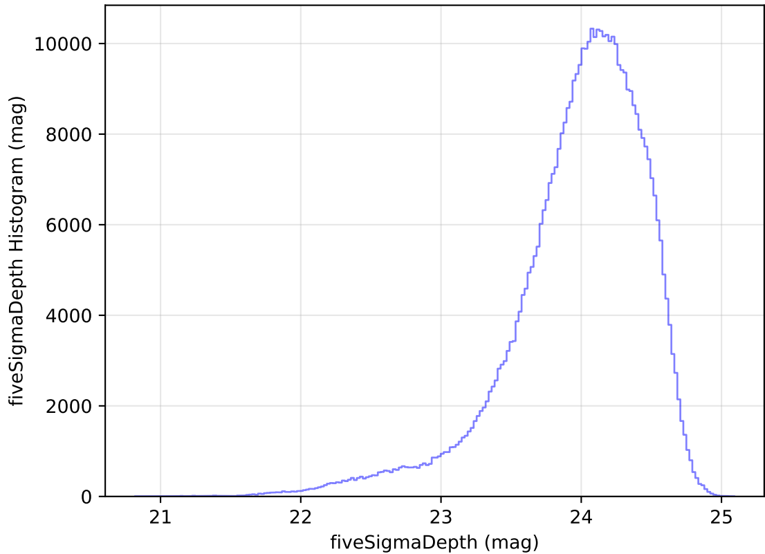
too_elab_heavy_r32_d2_griz_v3.4_10yrs All sky r band: fiveSigmaDepth Histogram
