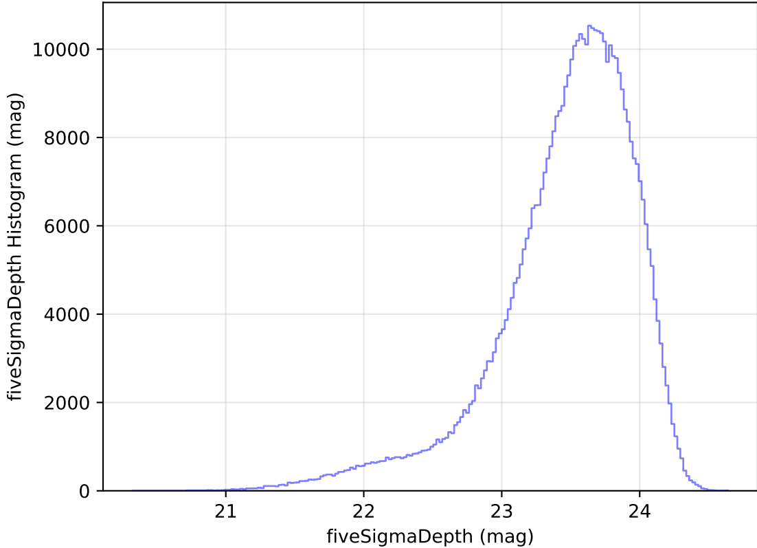
too_elab_heavy_r32_d2_griz_v3.4_10yrs All sky i band: fiveSigmaDepth Histogram
