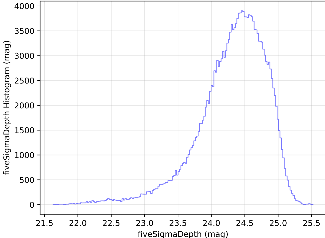
too_elab_heavy_r32_d2_griz_v3.4_10yrs All sky g band: fiveSigmaDepth Histogram
