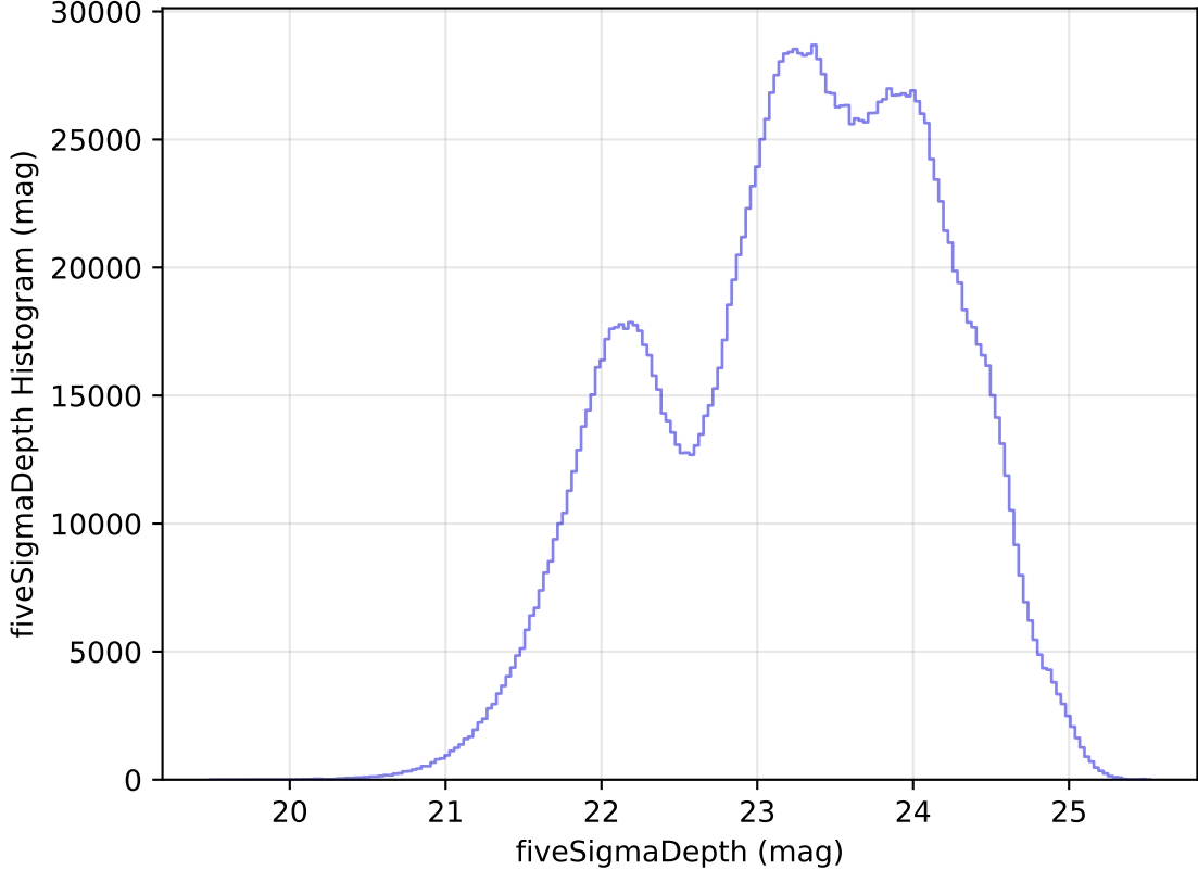
too_elab_heavy_r32_d2_griz_v3.4_10yrs All sky all bands: fiveSigmaDepth Histogram
