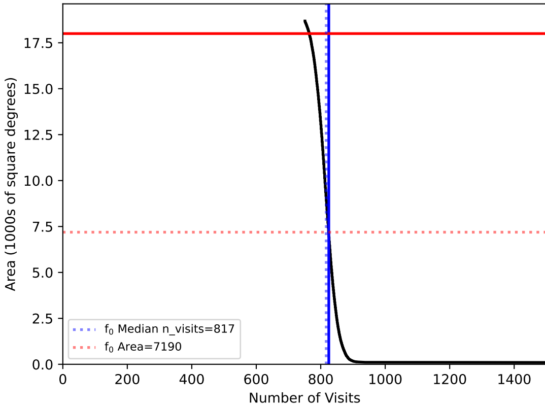
too_elab_heavy_r32_d2_griz_v3.4_10yrs WFD: f0
