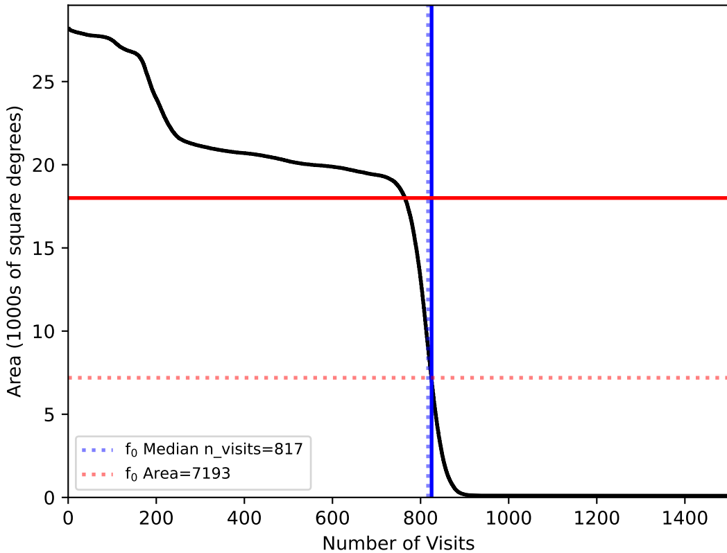
too_elab_heavy_r32_d2_griz_v3.4_10yrs All sky: f0
