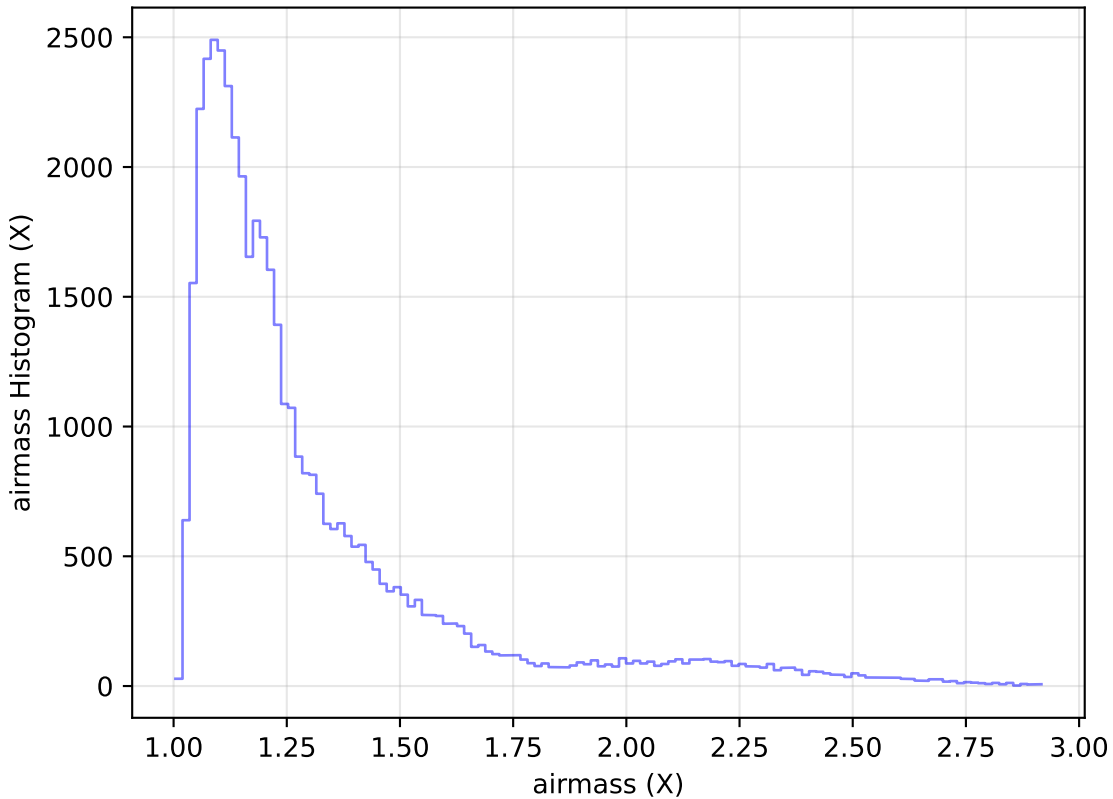
too_elab_heavy_r32_d2_griz_v3.4_10yrs Yr 1 z band: airmass Histogram
