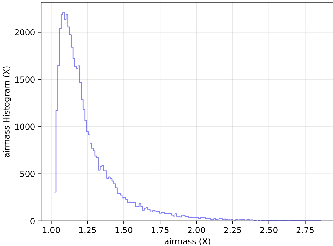
too_elab_heavy_r32_d2_griz_v3.4_10yrs Yr 1 y band: airmass Histogram
