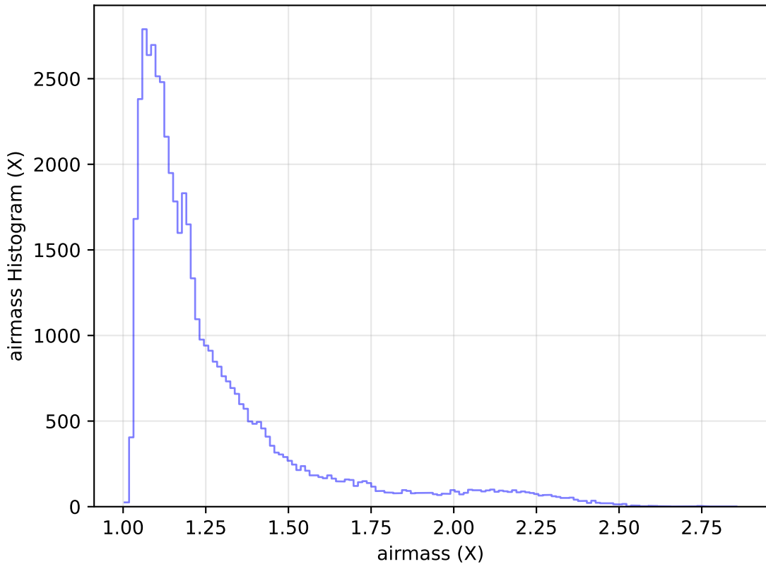
too_elab_heavy_r32_d2_griz_v3.4_10yrs Yr 1 r band: airmass Histogram
