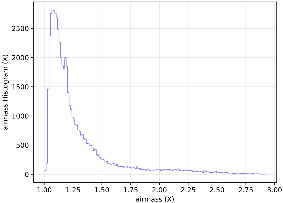
too_elab_heavy_r32_d2_griz_v3.4_10yrs Yr 1 i band: airmass Histogram
