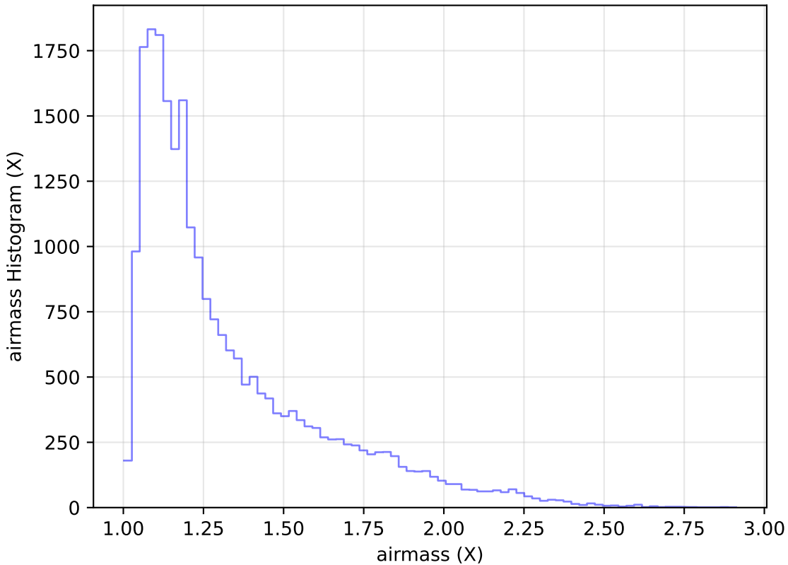
too_elab_heavy_r32_d2_griz_v3.4_10yrs Yr 1 g band: airmass Histogram
