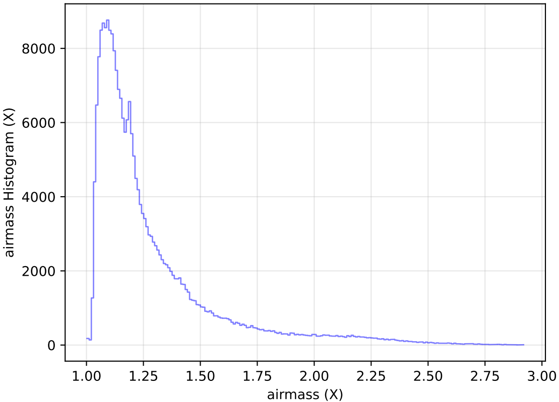
too_elab_heavy_r32_d2_griz_v3.4_10yrs Yr 1 all bands: airmass Histogram
