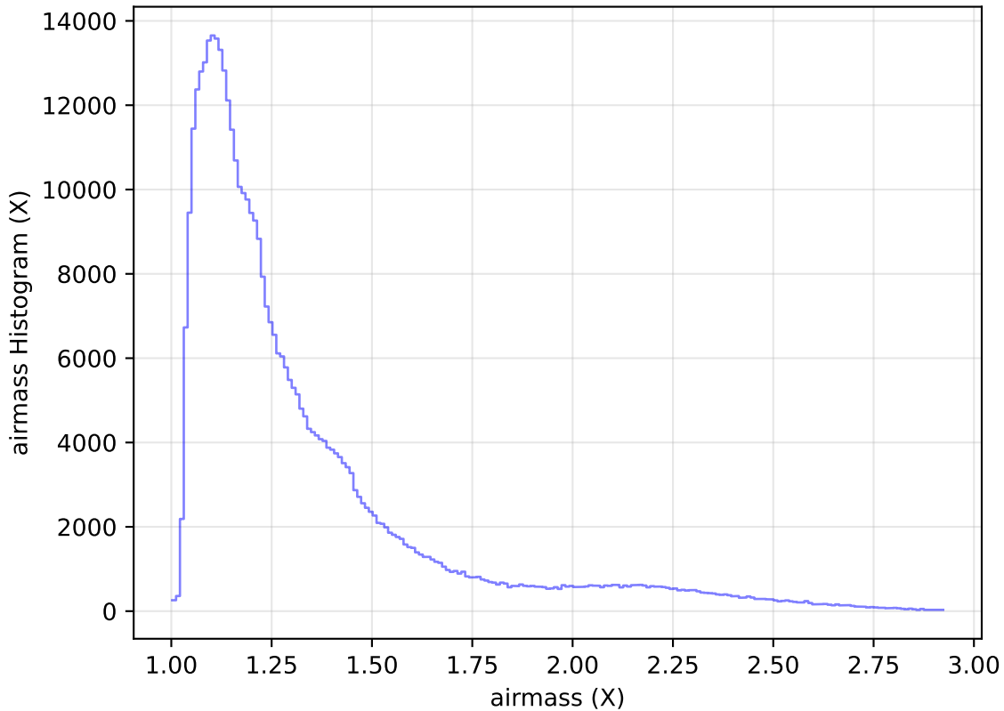
too_elab_heavy_r32_d2_griz_v3.4_10yrs WFD z band: airmass Histogram
