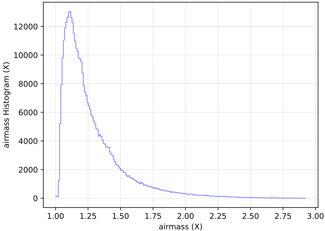
too_elab_heavy_r32_d2_griz_v3.4_10yrs WFD y band: airmass Histogram
