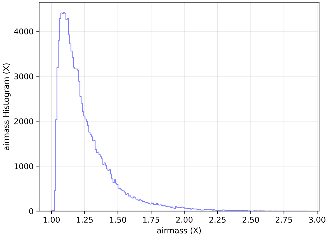
too_elab_heavy_r32_d2_griz_v3.4_10yrs WFD u band: airmass Histogram
