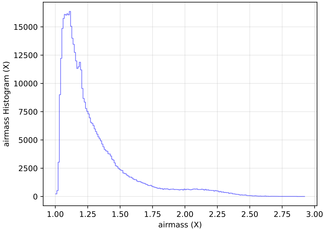
too_elab_heavy_r32_d2_griz_v3.4_10yrs WFD r band: airmass Histogram
