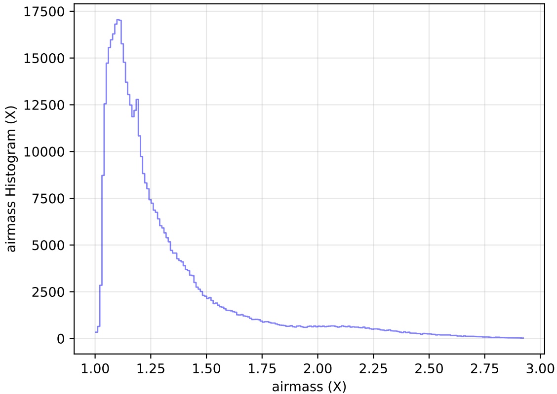
too_elab_heavy_r32_d2_griz_v3.4_10yrs WFD i band: airmass Histogram
