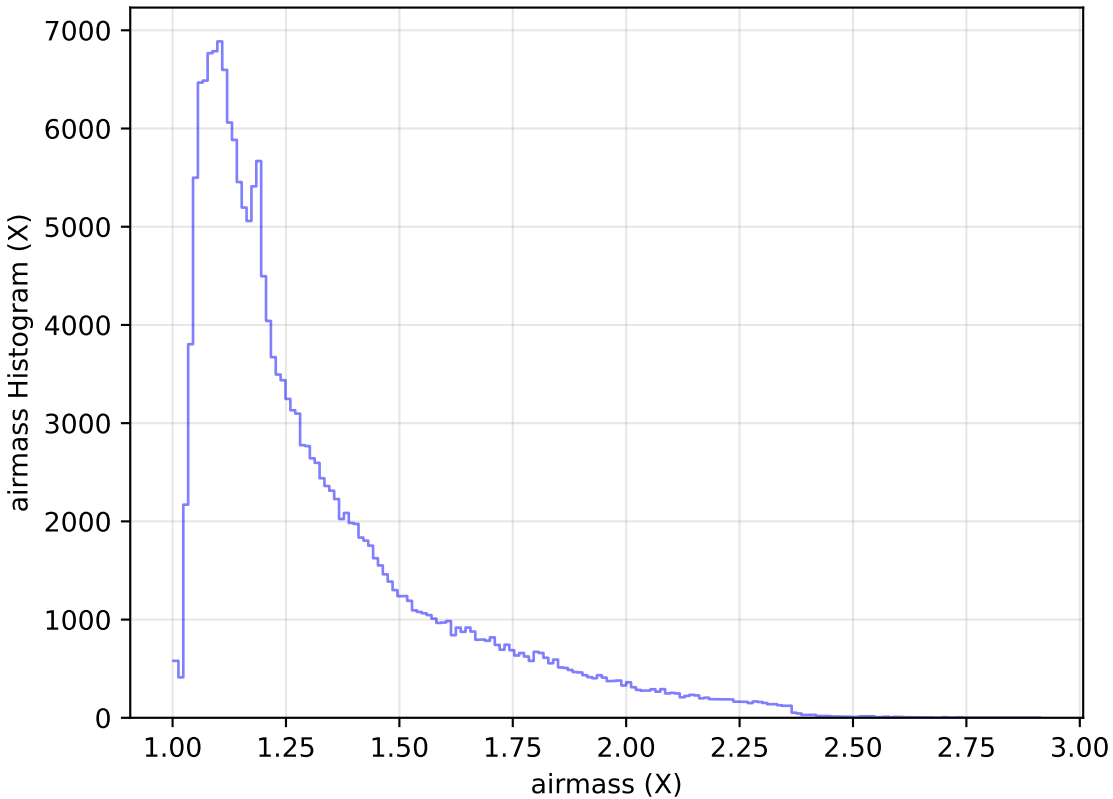
too_elab_heavy_r32_d2_griz_v3.4_10yrs WFD g band: airmass Histogram
