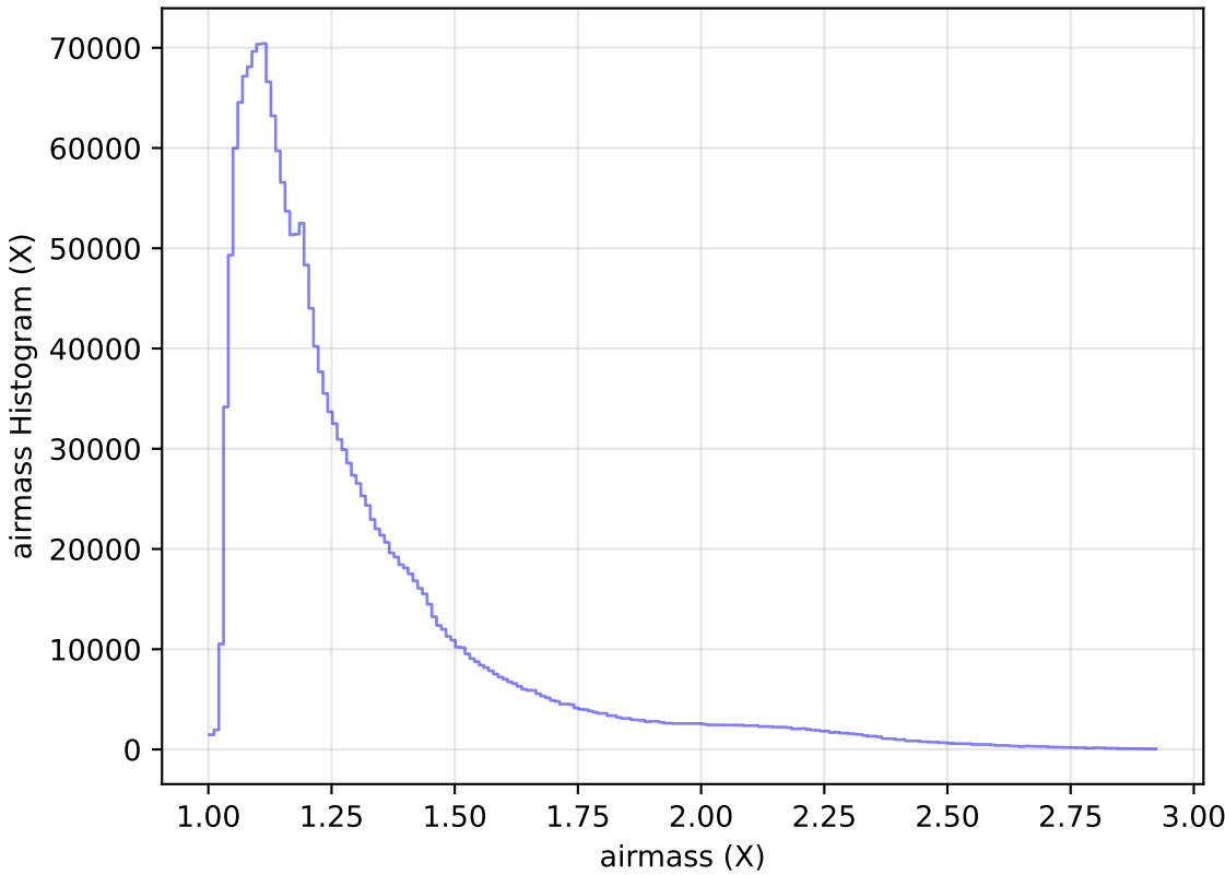
too_elab_heavy_r32_d2_griz_v3.4_10yrs WFD all bands: airmass Histogram
