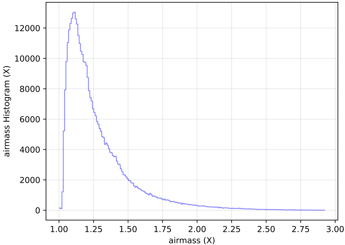
too_elab_heavy_r32_d2_griz_v3.4_10yrs All sky y band: airmass Histogram
