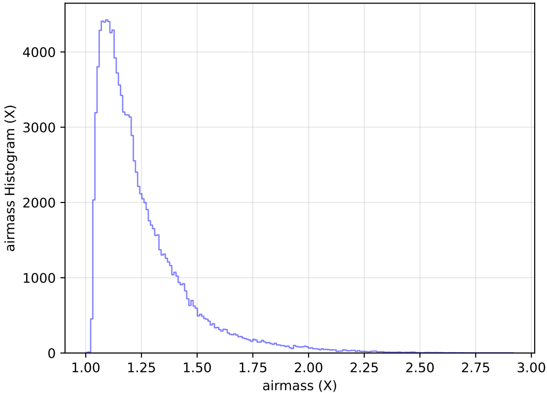
too_elab_heavy_r32_d2_griz_v3.4_10yrs All sky u band: airmass Histogram
