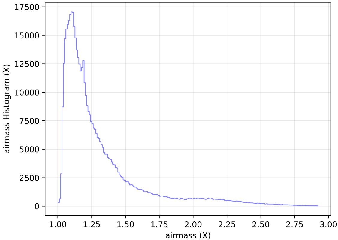
too_elab_heavy_r32_d2_griz_v3.4_10yrs All sky i band: airmass Histogram
