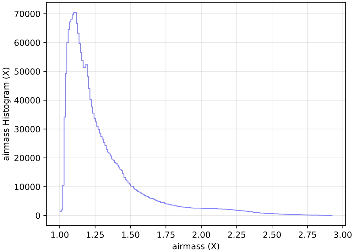
too_elab_heavy_r32_d2_griz_v3.4_10yrs All sky all bands: airmass Histogram
