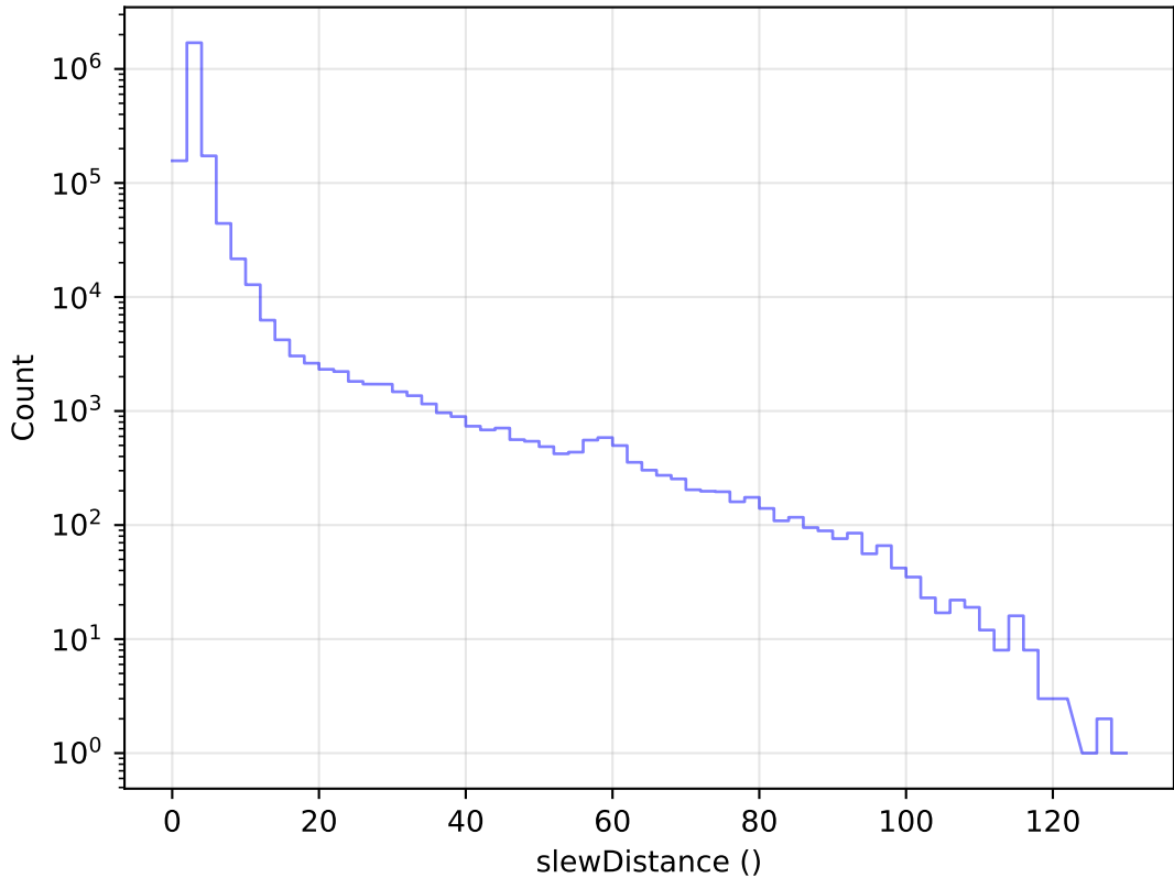
too_elab_heavy_r32_d2_griz_v3.4_10yrs All visits: Slew Distance Histogram
