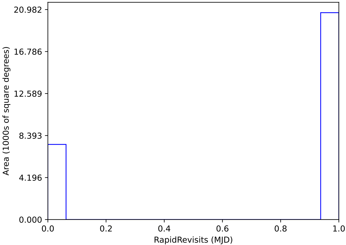
too_elab_heavy_r32_d2_griz_v3.4_10yrs All sky: RapidRevisits
