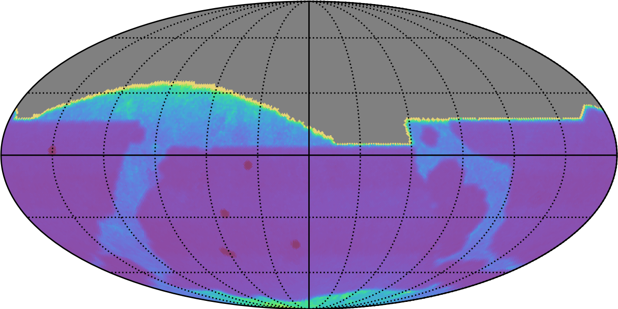
too_elab_heavy_r32_d2_griz_v3.4_10yrs All sky: Proper Motion Uncert @ 20.5
