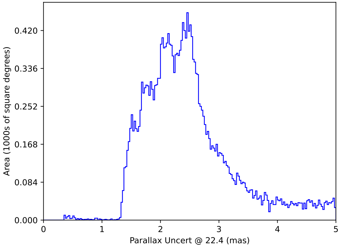
too_elab_heavy_r32_d2_griz_v3.4_10yrs All sky: Parallax Uncert @ 22.4
