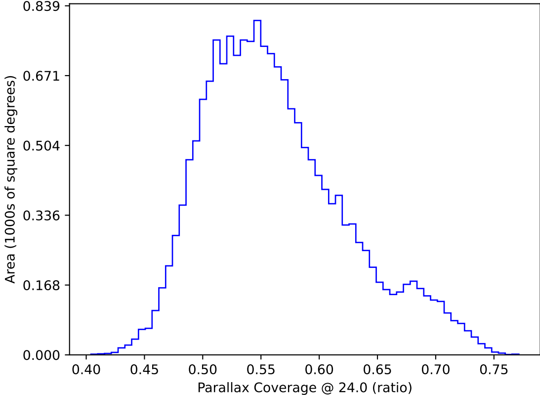
too_elab_heavy_r32_d2_griz_v3.4_10yrs WFD: Parallax Coverage @ 24.0
