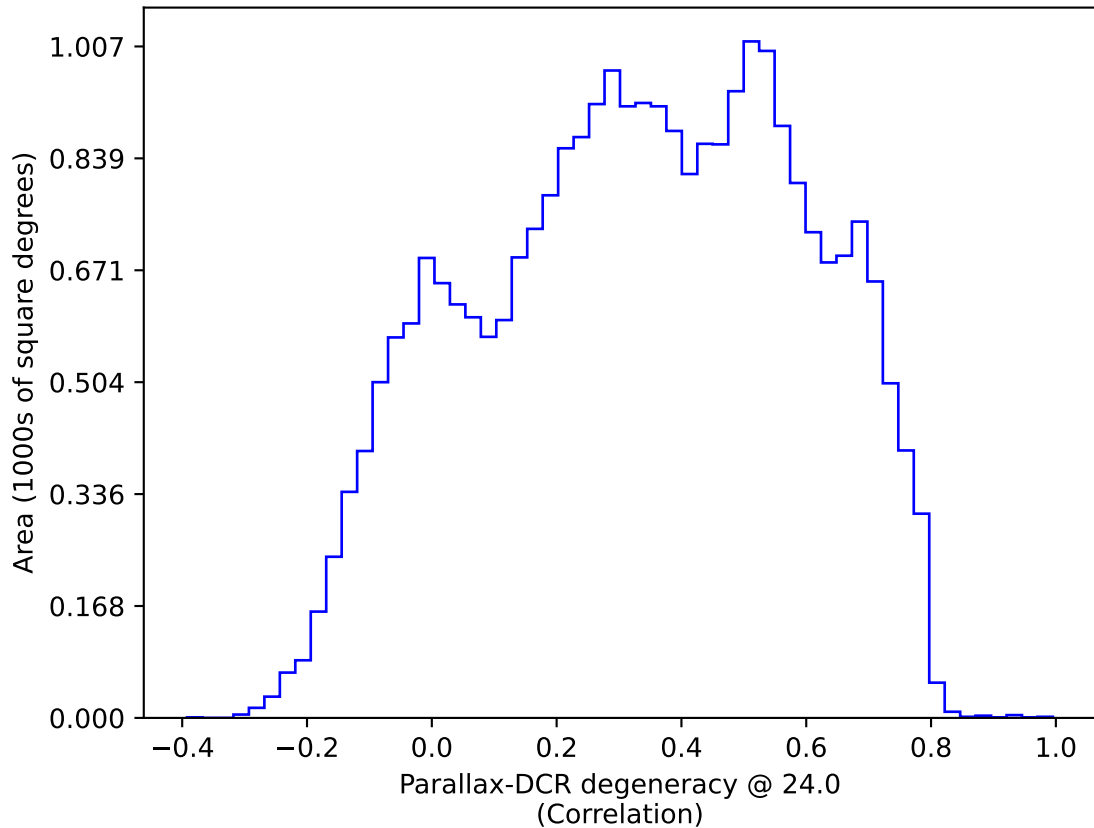
too_elab_heavy_r32_d2_griz_v3.4_10yrs All sky: Parallax-DCR degeneracy @ 24.0
