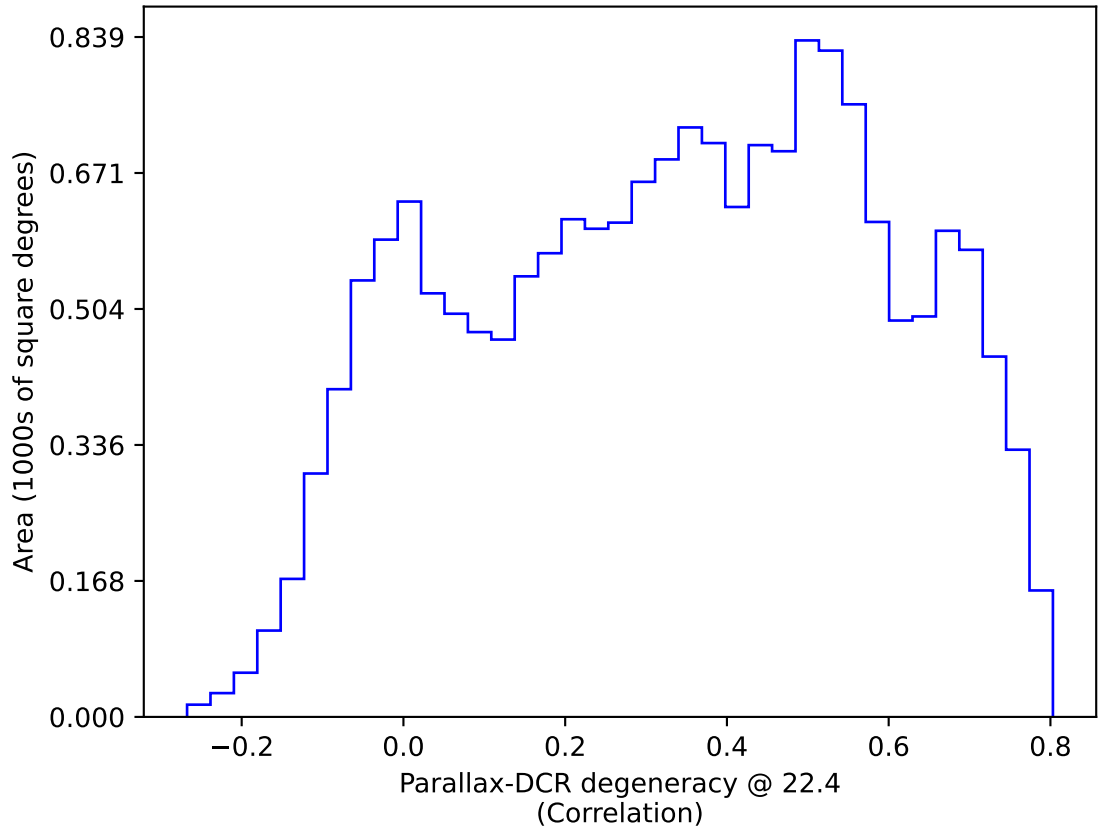
too_elab_heavy_r32_d2_griz_v3.4_10yrs WFD: Parallax-DCR degeneracy @ 22.4
