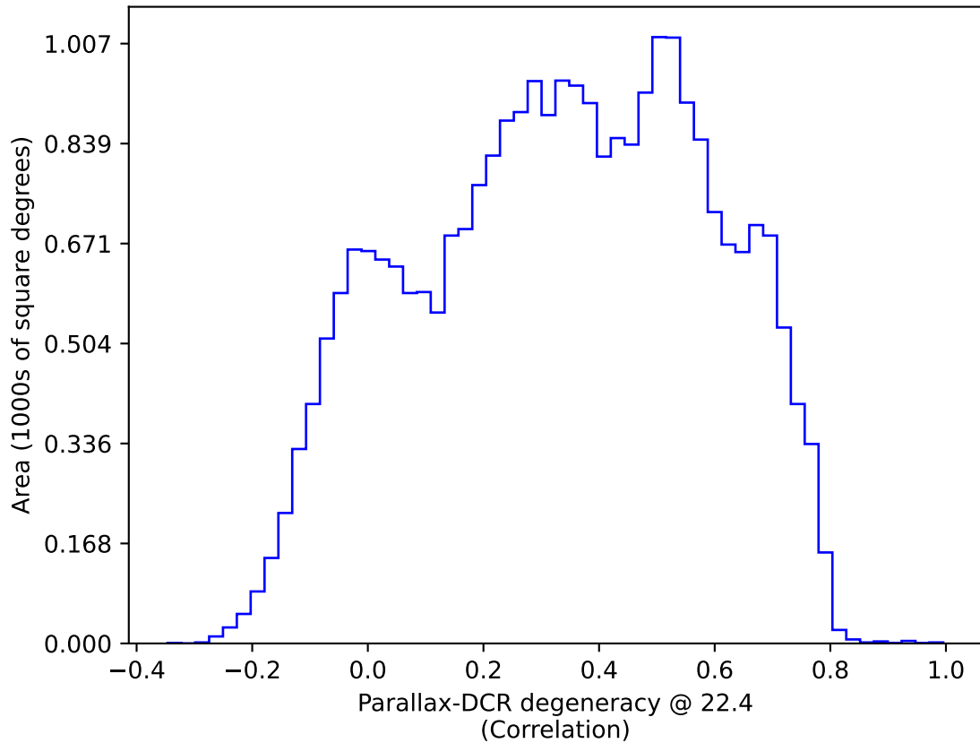
too_elab_heavy_r32_d2_griz_v3.4_10yrs All sky: Parallax-DCR degeneracy @ 22.4
