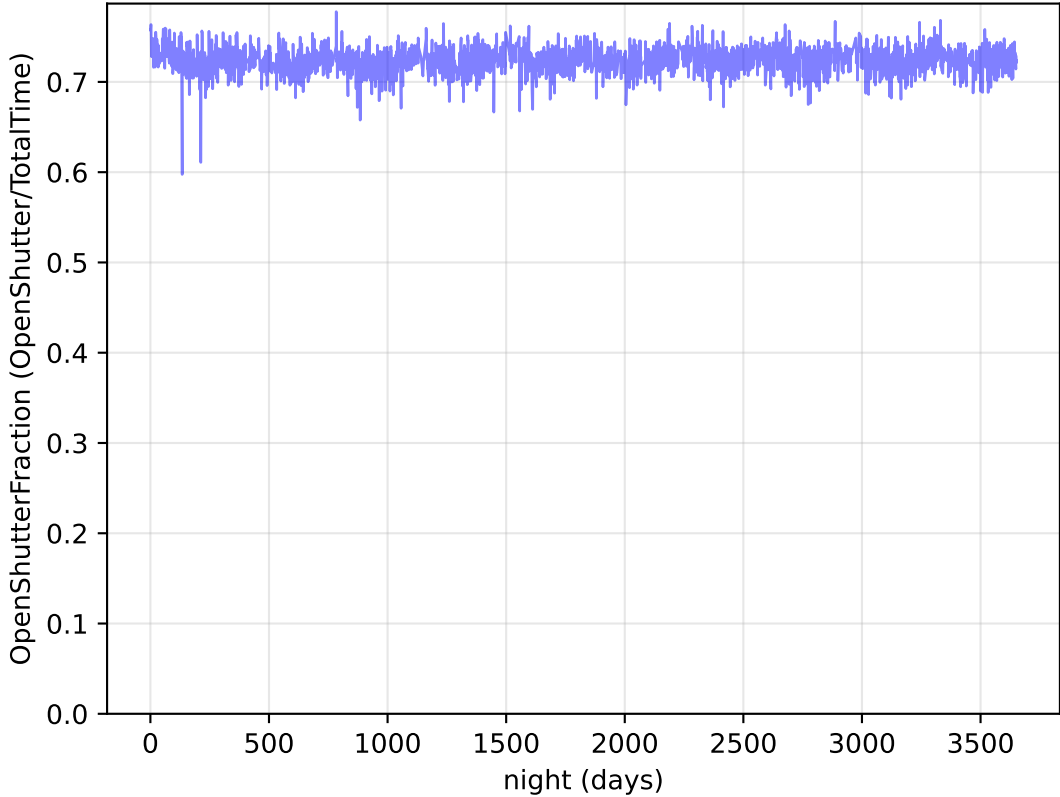
too_elab_heavy_r32_d2_griz_v3.4_10yrs Per night: OpenShutterFraction
