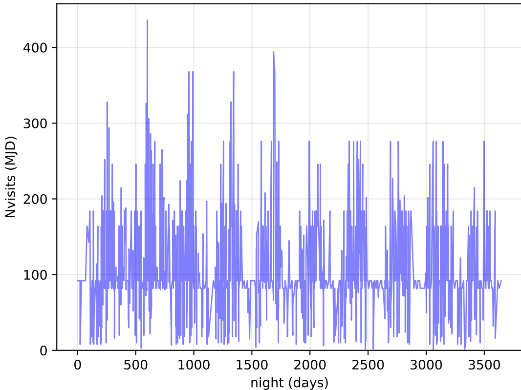
too_elab_heavy_r32_d2_griz_v3.4_10yrs DDF: Nvisits
