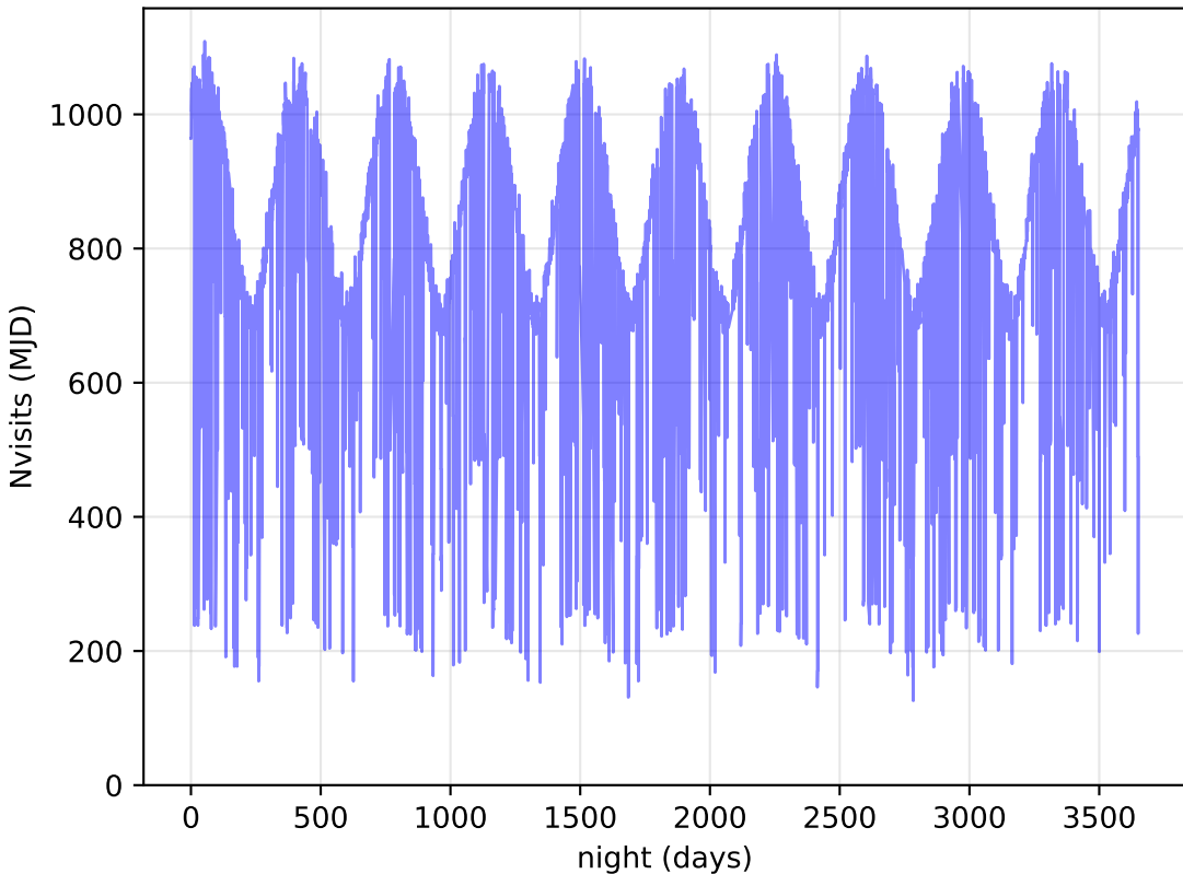
too_elab_heavy_r32_d2_griz_v3.4_10yrs All visits: Nvisits
