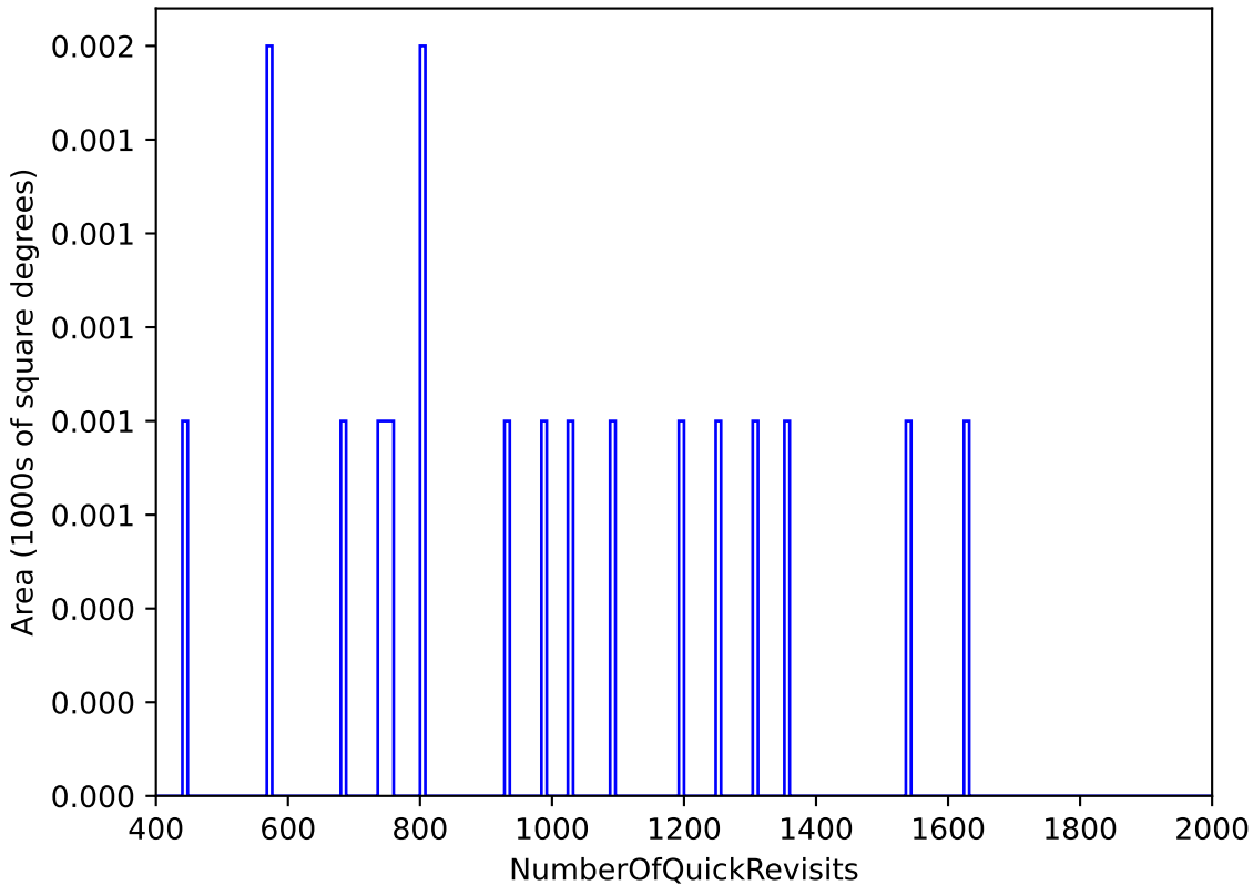
too_elab_heavy_r32_d2_griz_v3.4_10yrs WFD: NumberOfQuickRevisits
