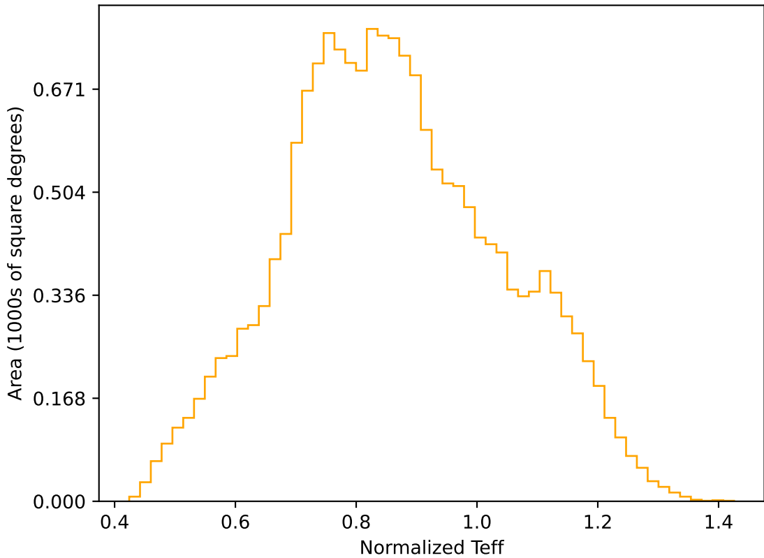
too_elab_heavy_r32_d2_griz_v3.4_10yrs WFD r band: Normalized Teff
