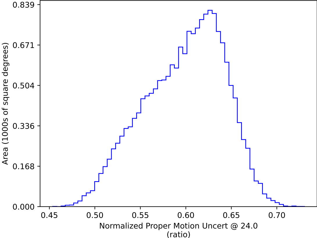
too_elab_heavy_r32_d2_griz_v3.4_10yrs WFD: Normalized Proper Motion Uncert @ 24.0
