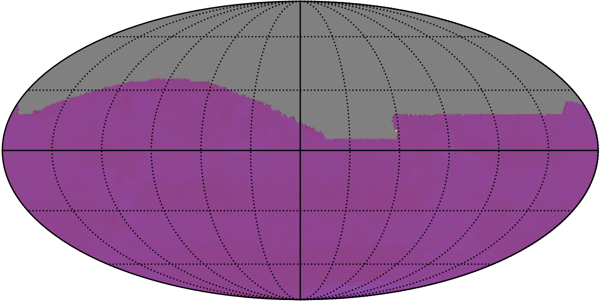
too_elab_heavy_r32_d2_griz_v3.4_10yrs All sky: Normalized Proper Motion Uncert @ 24.0
