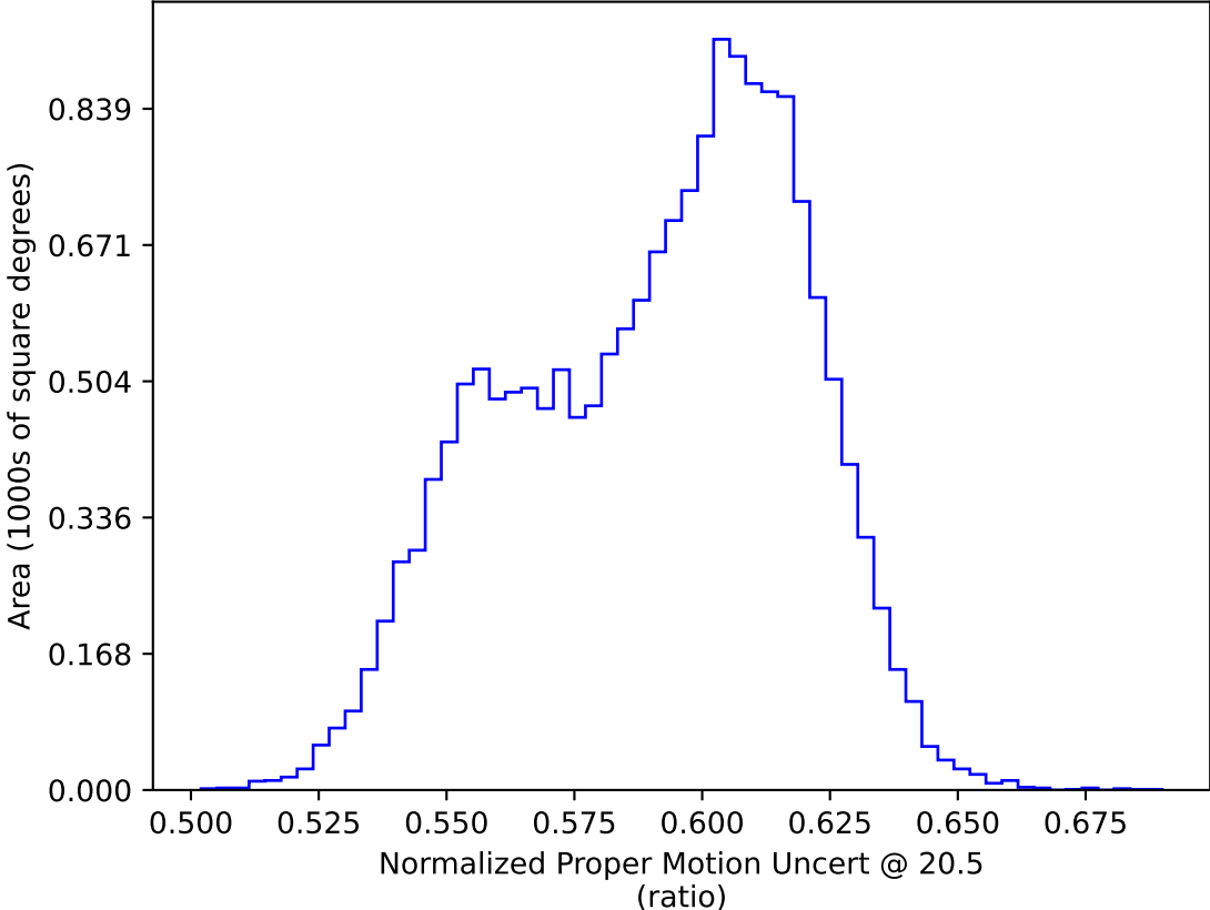
too_elab_heavy_r32_d2_griz_v3.4_10yrs WFD: Normalized Proper Motion Uncert @ 20.5
